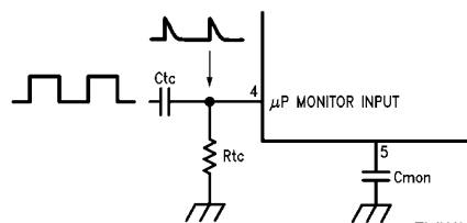
FIGURE 2. Monitoring Square Wave \mu\text{P} Signals
