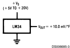
FIGURE 1. Basic Fahrenheit Temperature Sensor (+5° to +300°F)
