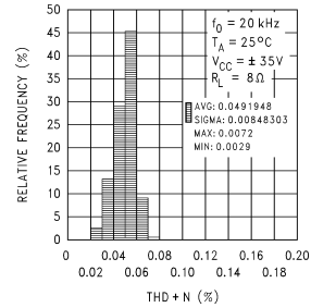
THD+N Distribution
