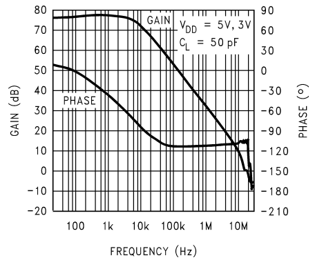
Amplifier Open Loop vs Frequency Respose
