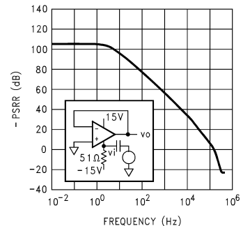
Negative Power Supply Voltage Rejection Ratio
