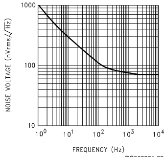
Op Amp Voltage Noise vs Frequency
