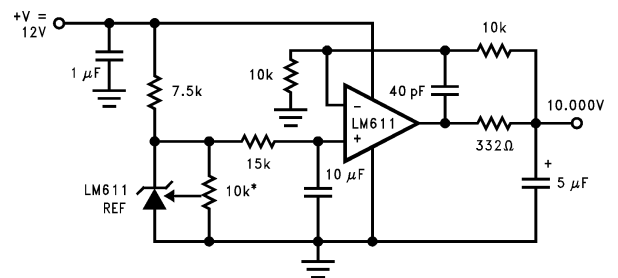
FIGURE 12. Ultra Low Noise 10.000V Reference. Total Output Noise is Typically 14 \mu\text{V}_{RMS} . Adjust the 10k pot for 10.000V.
