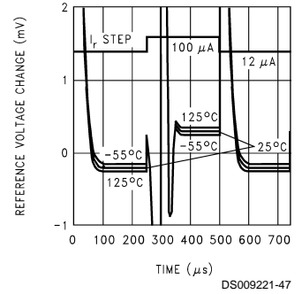
Reference Voltage with 100–12 μA Current Step
