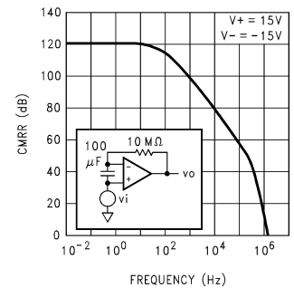
Common-Mode Input Voltage Rejection Ratio
