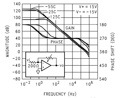
Small-Signal Voltage Gain vs Frequency and Temperature
