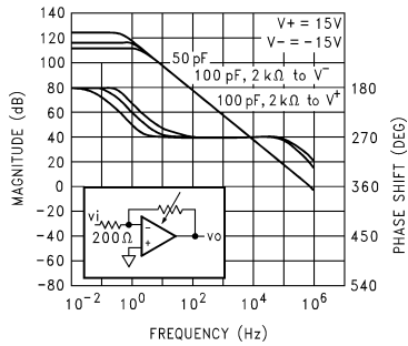
Small-Signal Voltage Gain vs Frequency and Load
