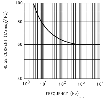
Op Amp Current Noise vs Frequency
