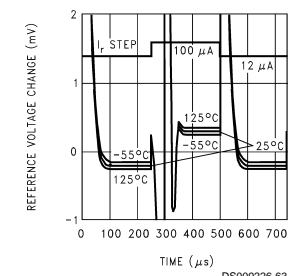
Reference Voltage with 100 ~ 12 µA Current Step
