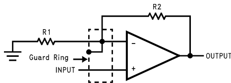
Non-Inverting Amplifier
