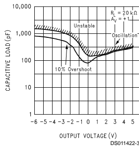
Stability vs Capacitive Load, R_L = 20\text{ k}\Omega
