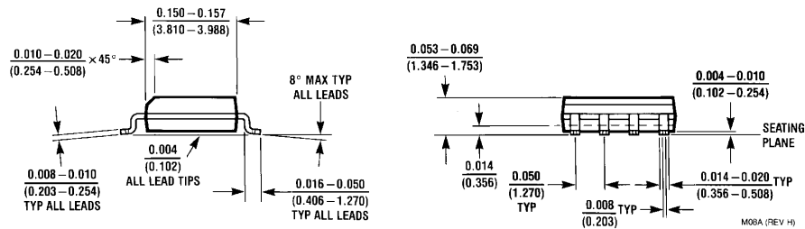
8-Pin Small Outline Package Order Number LMC6061AIM or LMC6061IM NS Package Number M08A
