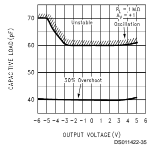
Stability vs Capacitive Load R_L = 1\text{ M}\Omega
