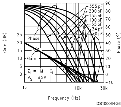
Open Loop Gain/Phase vs Frequency For Various C_L ( Z_L = 1 M\Omega \parallel C_L )
