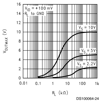
Maximum Output Voltage vs Load Resistance
