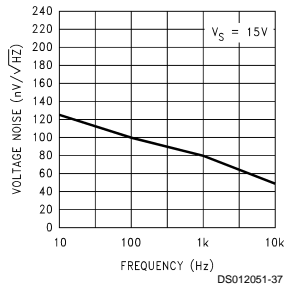
Input Voltage Noise vs Frequency
