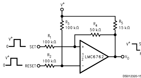
FIGURE 7. Bi-Stable Multivibrator
