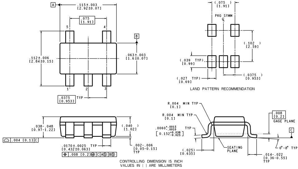
5-Pin SOT23 NS Product Number MF05A
