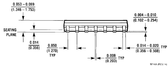
14-Pin SOIC NS Product Number M14A
