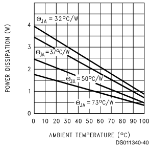
Maximum Power Dissipation (TO-263) (Note 2)
