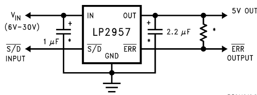
LP2957 Basic Application
