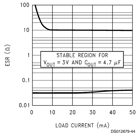
FIGURE 2. 3V/4.7 \mu\text{F} ESR Curves
