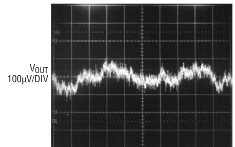
C_{OUT} = 10\mu F I_L = 500mA 1763 G44
