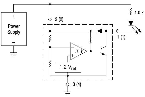
Figure 16. Voltage Monitor
