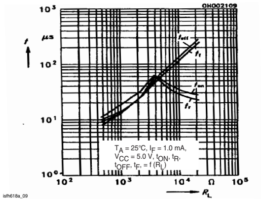
Figure 10. Switching times (typ.)
