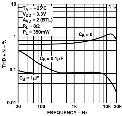
Figure 10. THD+N vs. Frequency
