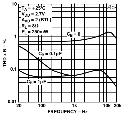
Figure 16. THD+N vs. Frequency
