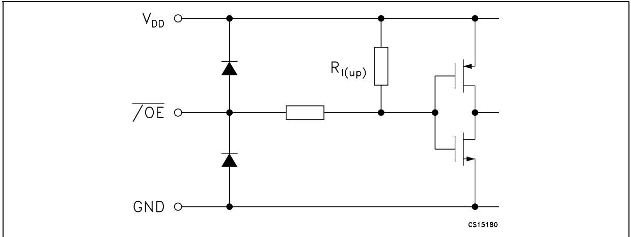
Figure 2: \overline{OE} Terminal
