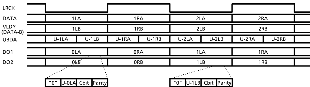
Figure 4b Data Input/Output Format Example 2 ((M2, M1) = (L, H) ; 2ch x 2 input, 2ch x 2 output mode)
