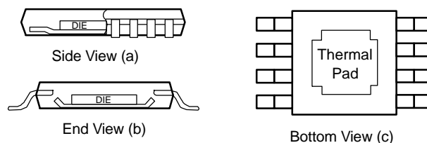
Figure 111. Views of Thermally Enhanced Package
