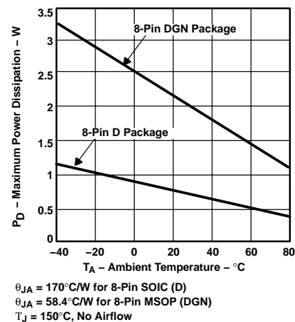
Figure 113. Maximum Power Dissipation vs Ambient Temperature
