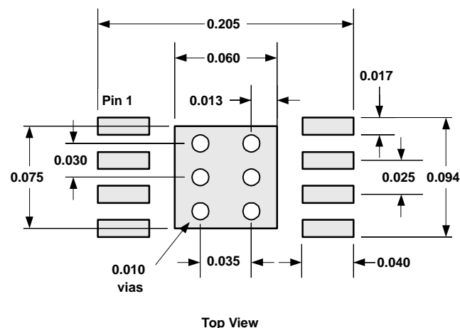
Figure 112. PowerPAD PCB Etch and Via Pattern
