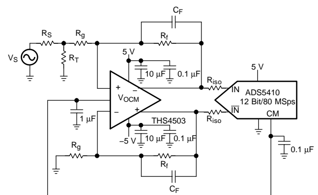
Using the THS4503 With the ADS5410 Figure 97
