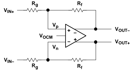
Diagram For Input Common-Mode Range Equations Figure 95
