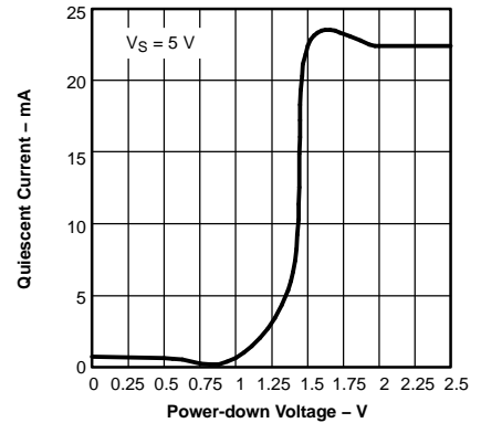
QUIESCENT CURRENT VS POWER-DOWN VOLTAGE
