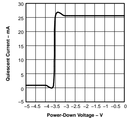
QUIESCENT CURRENT VS POWER-DOWN VOLTAGE
