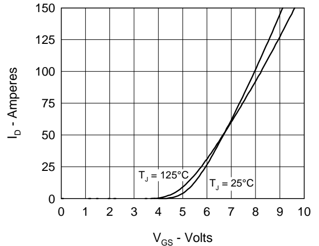
Fig. 2 Input Admittance
