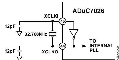
Figure 76. External Parallel Resonant Crystal Connections
