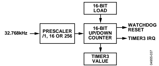
Figure 65. Timer3 Block Diagram
