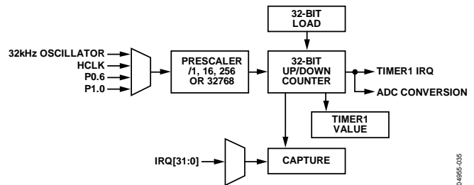
Figure 63. Timer1 Block Diagram
