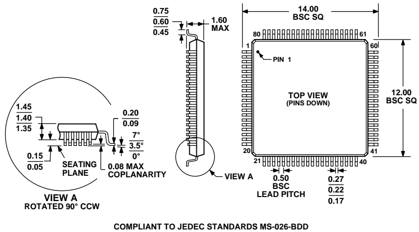
Figure 83. 80-Lead Low Profile Quad Flat Package [LQFP] (ST-80-1) Dimensions shown in millimeters
