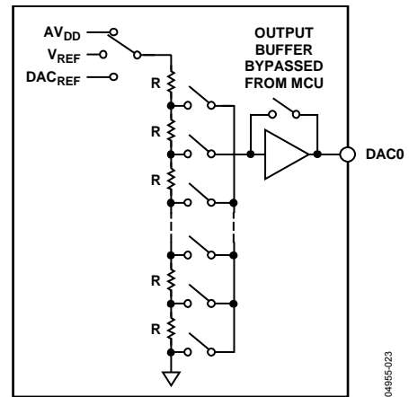
Figure 50. DAC Structure
