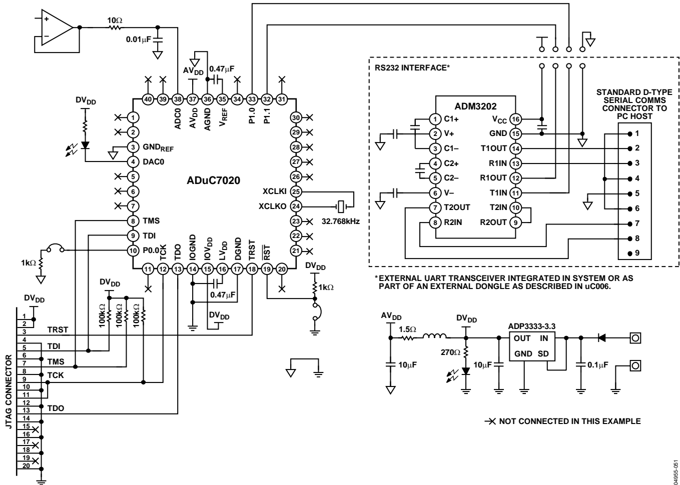
Figure 79. Typical System Configuration
