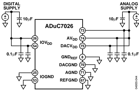
Figure 72. External Dual Supply Connections
