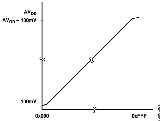
Figure 51. Endpoint Nonlinearities Due to Amplifier Saturation
