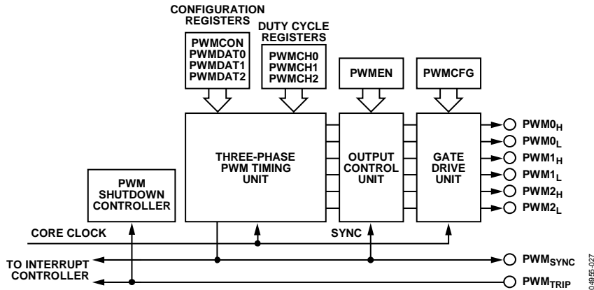
Figure 55. Overview of the PWM Controller
