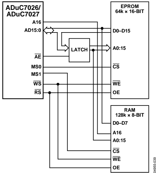
Figure 67. Interfacing to External EPROM/RAM
