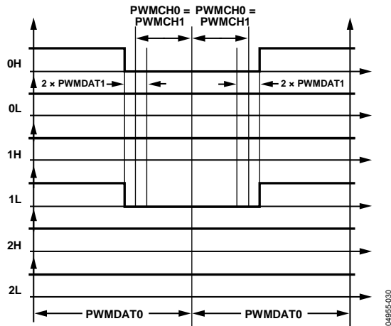
Figure 58. Active LO PWM Signals Suitable for ECM Control, PWMCH0 = PWMCH1 , Crossover 1H/1L Pair and Disable 0L, 1H, 2H, and 2L Outputs in Single Update Mode.
