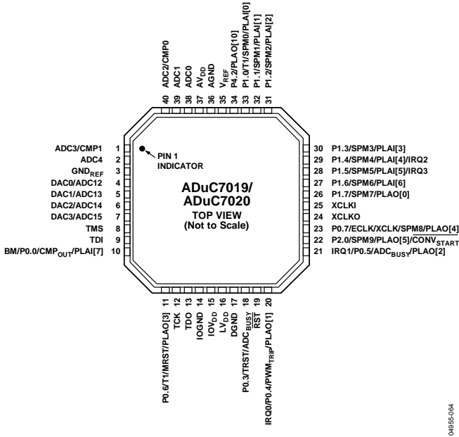
Figure 10. ADuC7019/ADuC7020 Pin Configuration
