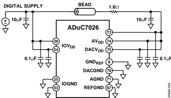
Figure 73. External Single Supply Connections
