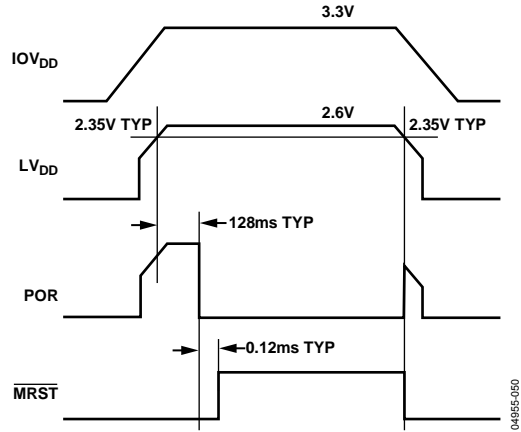
Figure 78. ADuC7019/20/21/22/24/25/26/27 Internal Power-on Reset Operation
