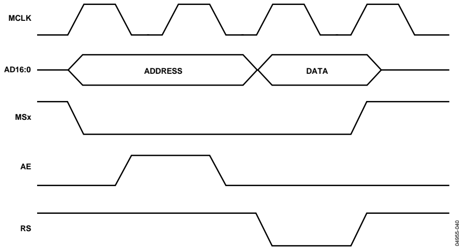
Figure 68. External Memory Read Cycle
