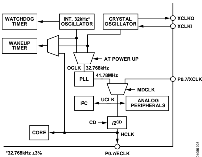
Figure 54. Clocking System
