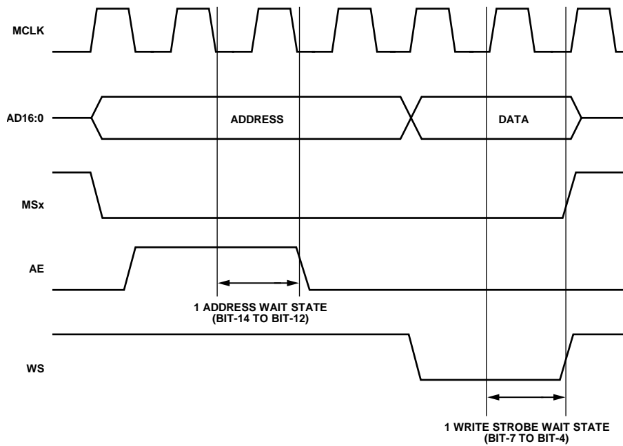
Figure 71. External Memory Write Cycle with Wait States
