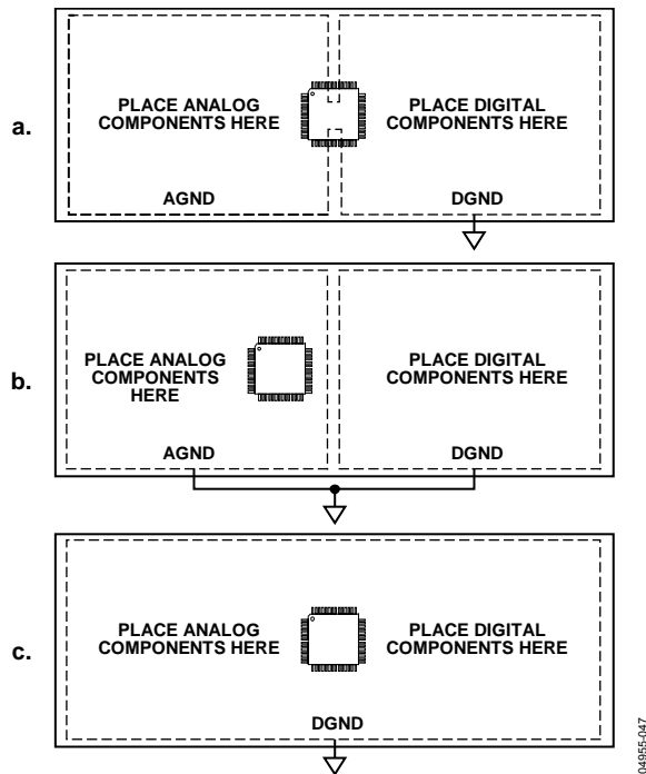
Figure 75. System Grounding Schemes
