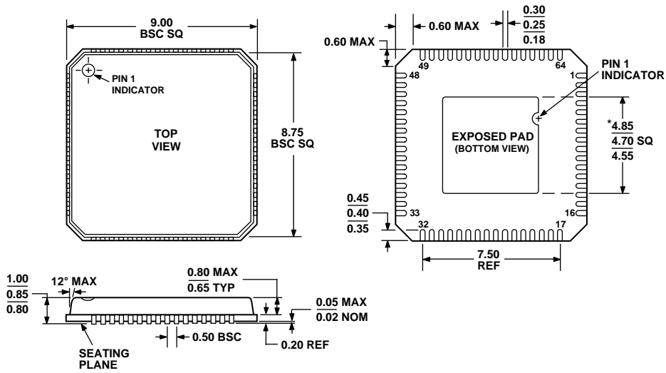
Figure 81. 64-Lead Frame Chip Scale Package [LFCSP_VQ] 9 mm x 9 mm Body, Very Thin Quad (CP-64-1) Dimensions shown in millimeters
