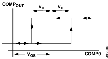
Figure 53. Comparator Hysteresis Transfer Function
