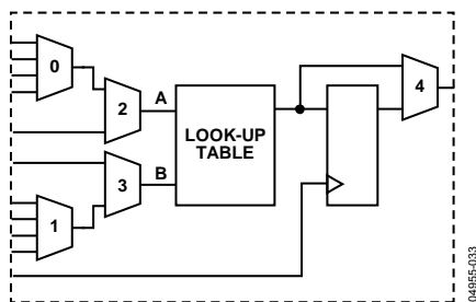
Figure 61. PLA Element
