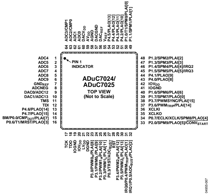
Figure 13. ADuC7024/ADuC7025 64-Lead CSP Pin Configuration
