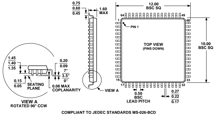
Figure 82. 64-Lead Low Profile Quad Flat Package [LQFP] (ST-64-2) Dimensions shown in millimeters
