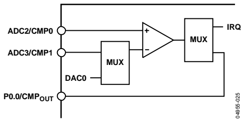
Figure 52. Comparator
