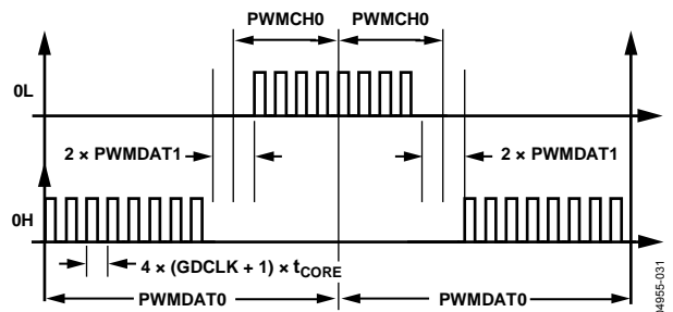
Figure 59. Typical PWM Signals with High Frequency Gate Chopping Enabled on Both High-Side and Low-Side Switches
