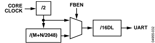
Figure 60. Baud Rate Generation Options
