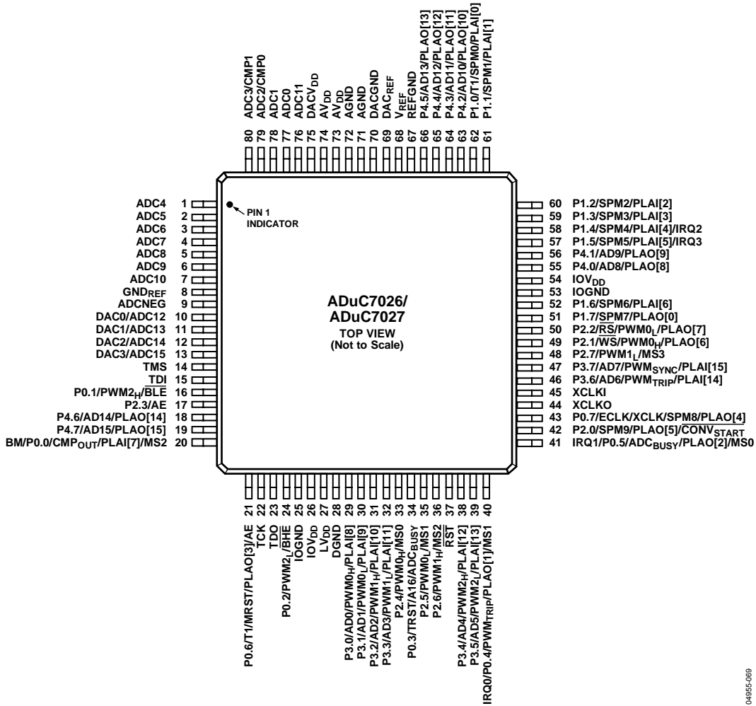
Figure 15. ADuC7026/ADuC7027 Pin Configuration
