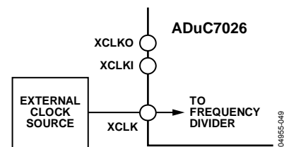
Figure 77. Connecting an External Clock Source
