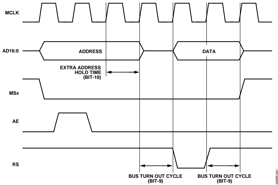
Figure 69. External Memory Read Cycle with Address Hold and Bus Turn Cycles
