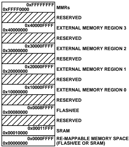
Figure 33. Physical Memory Map
