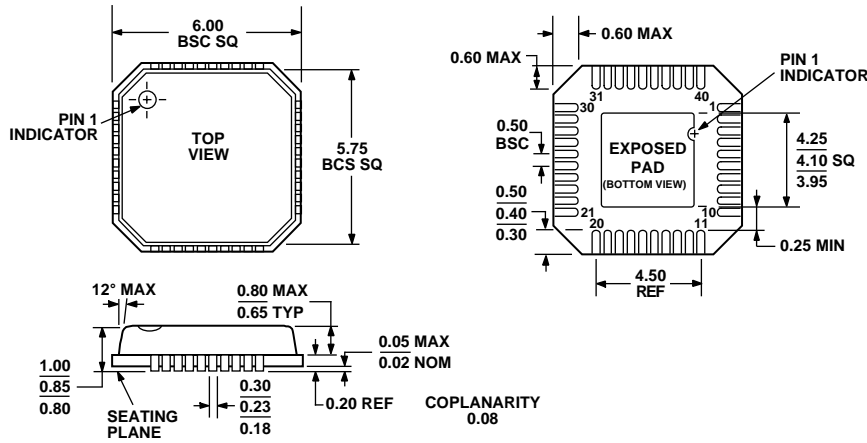
Figure 80. 40-Lead Frame Chip Scale Package [LFCSP_VQ] 6 mm x 6 mm Body, Very Thin Quad (CP-40) Dimensions shown in millimeters
