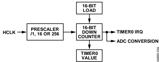
Figure 62. Timer0 Block Diagram
