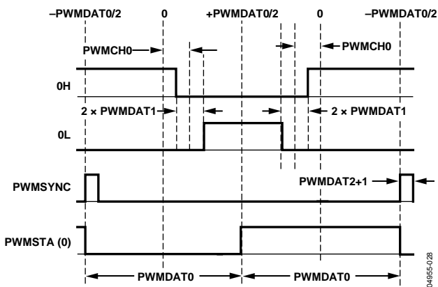
Figure 56. Typical PWM Outputs of Three-Phase Timing Unit in Single Update Mode
