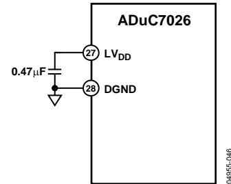
Figure 74. Voltage Regulator Connections
