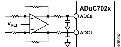
Figure 48. Buffering Differential Inputs
