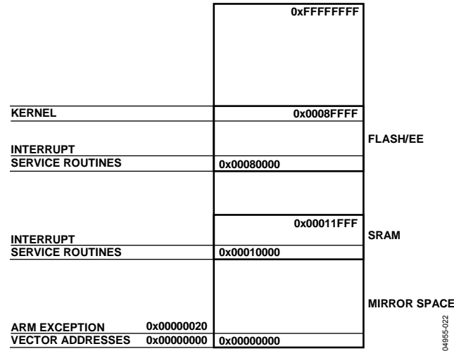
Figure 49. Remap for Exception Execution
