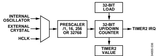
Figure 64. Timer2 Block Diagram
