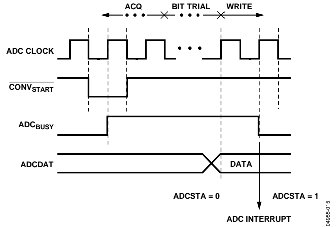
Figure 40. ADC Timing
