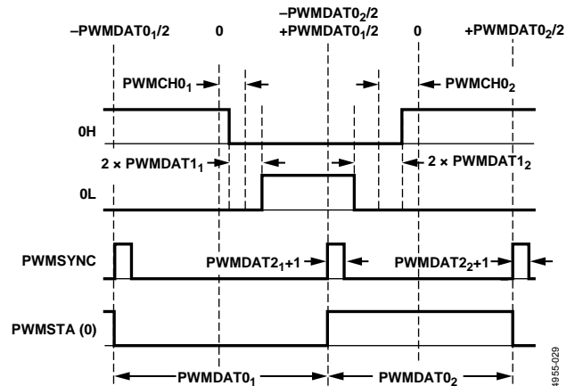
Figure 57. Typical PWM Outputs of the Three-Phase Timing Unit in Double Update Mode
