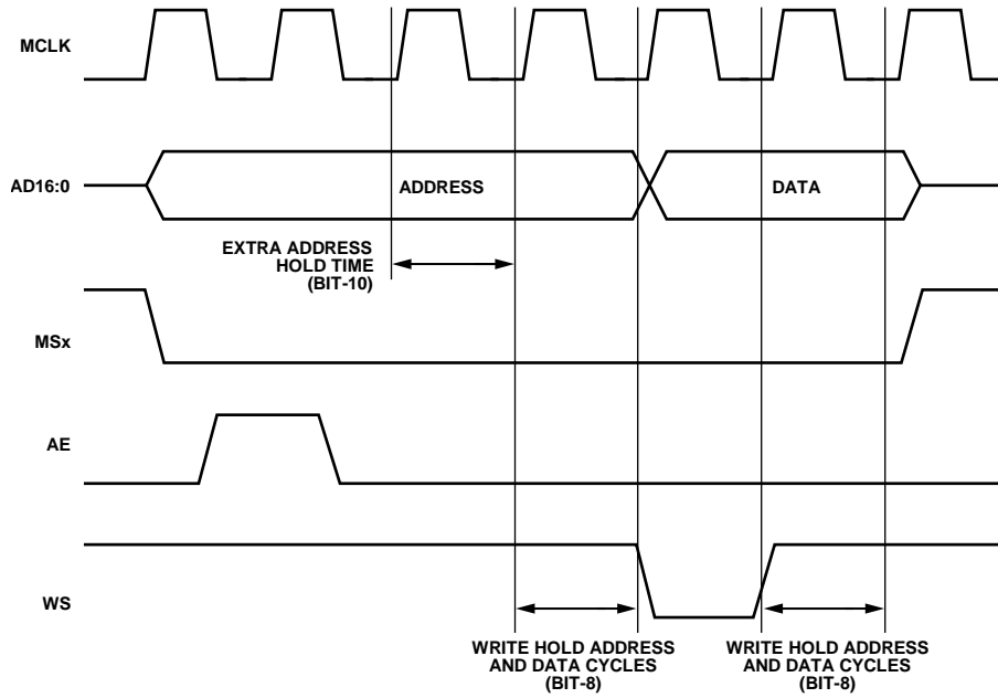
Figure 70. External Memory Write Cycle with Address and Write Hold Cycles
