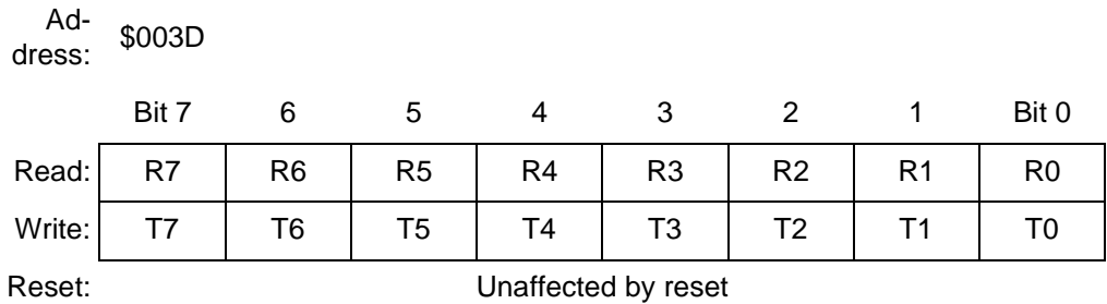
Figure 13-13. SCI Data Register (SCDR)
