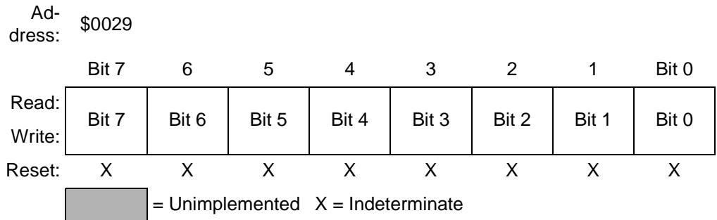
Figure 9-32. PWM Counter Modulo Register Low (PDMODL)
