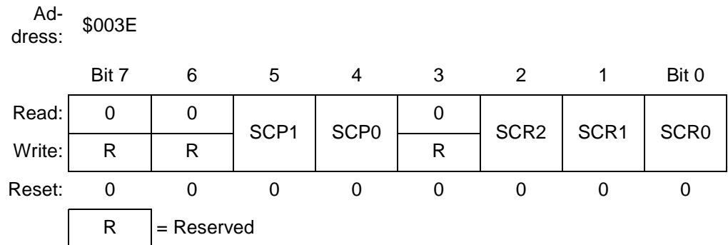
Figure 13-14. SCI Baud Rate Register (SCBR)
