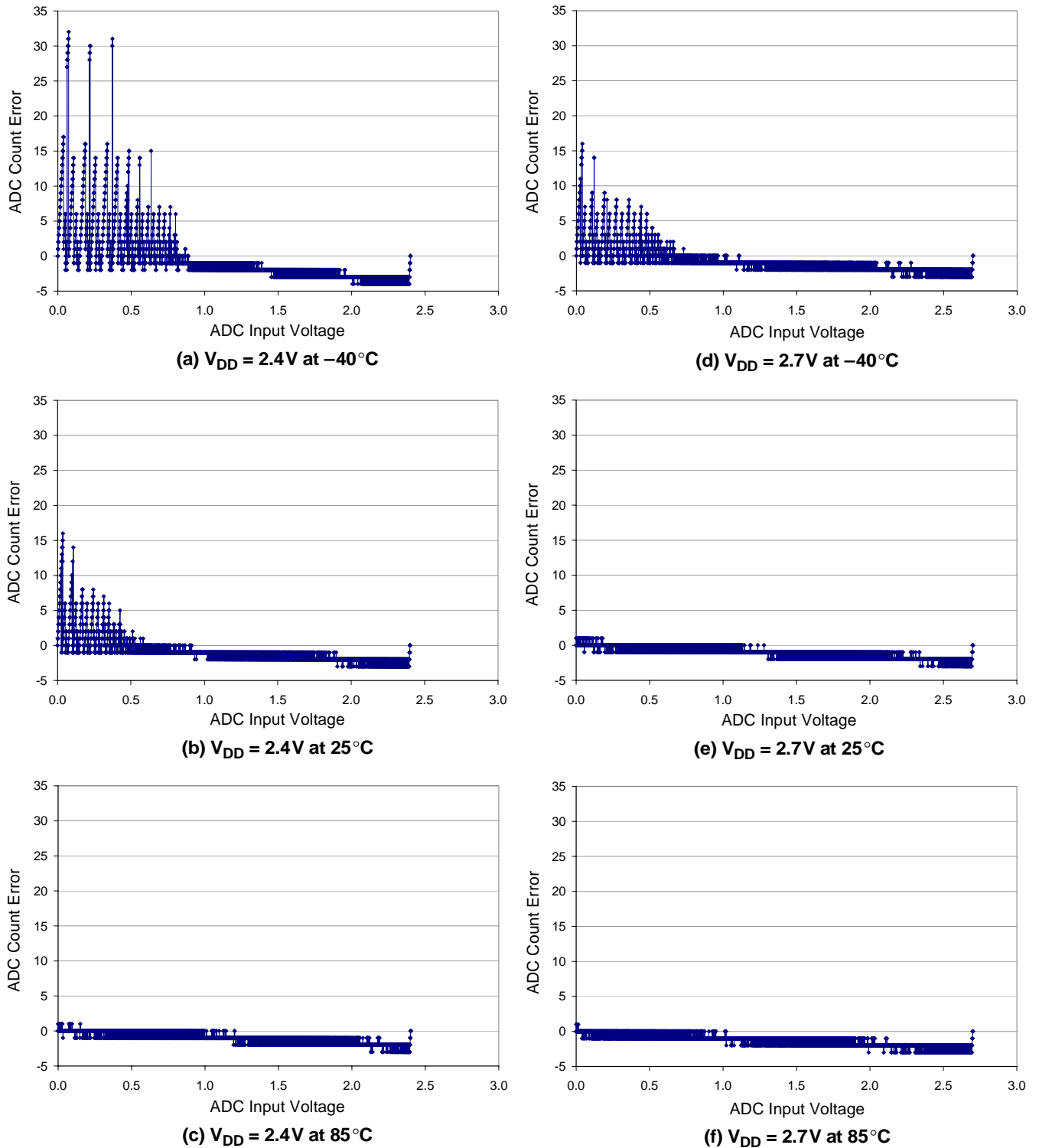
Figure 2. Typical ADC Accuracy (2.4V and 2.7V)
