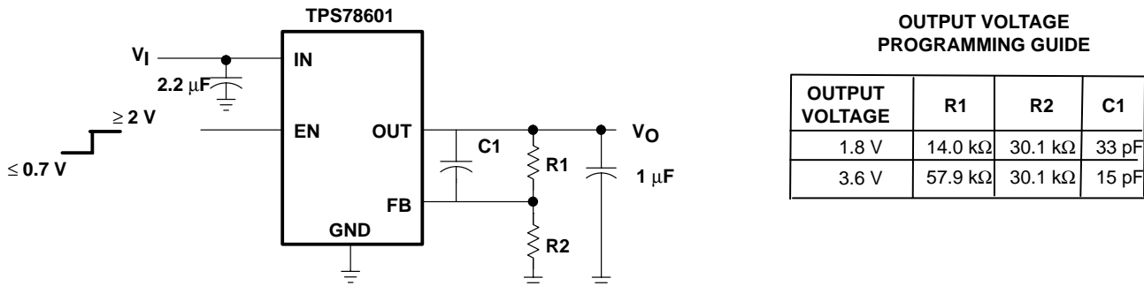
Figure 25. TPS78601 Adjustable LDO Regulator Programming
