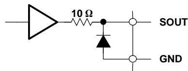
Figure 2. Output Equivalent Circuit
