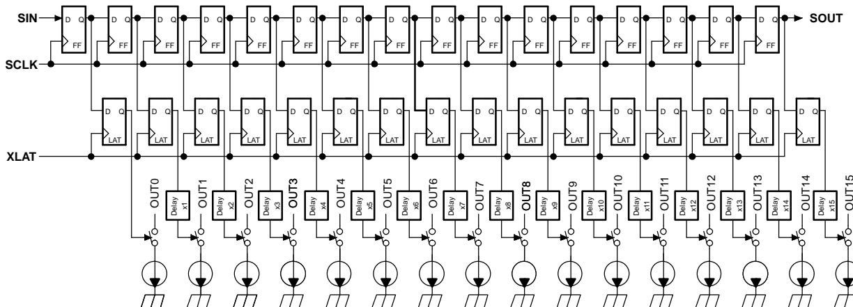
Figure 7. Shift Register and Data Latch for ON/OFF Setting
