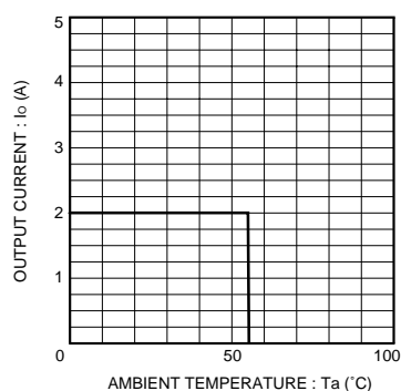
Fig.6 Derating curve
