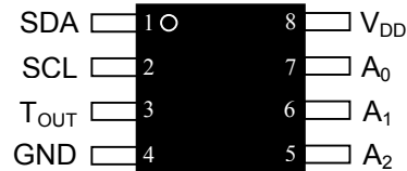
\mu\text{SOP} (DS1631U, DS1631AU, DS1731U)
