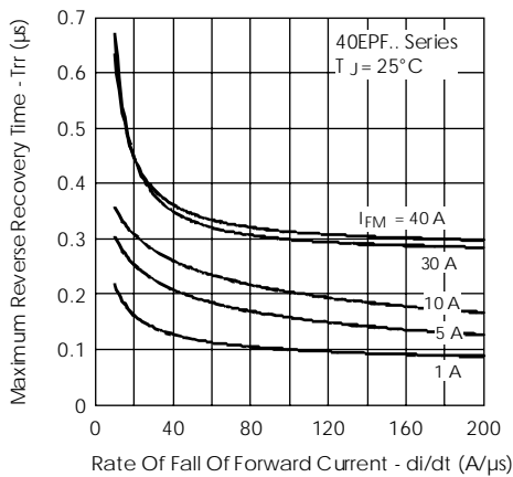
Fig.8- Recovery Time Characteristics, T J =25°C
