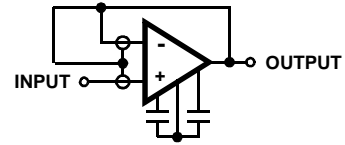
FIGURE 1B. FOLLOWER
