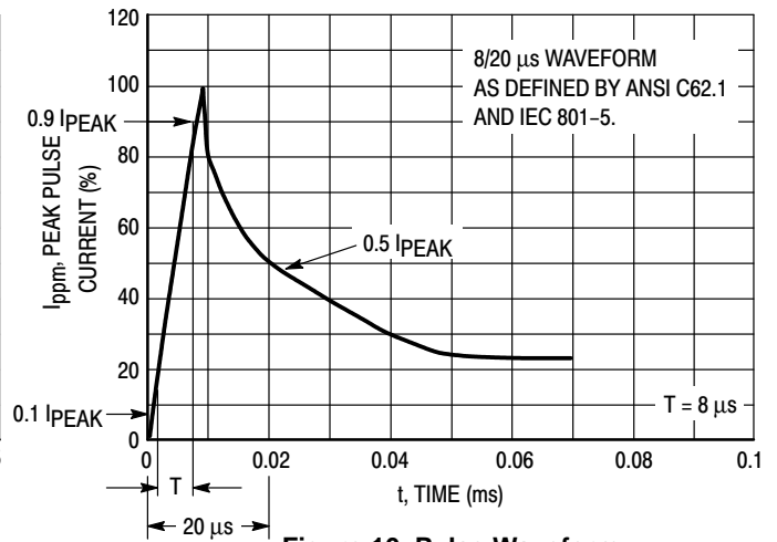
Figure 10. Pulse Waveform
