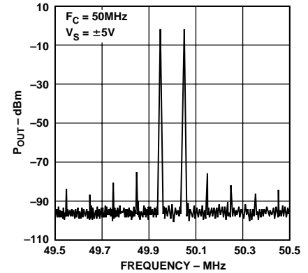
Figure 16. Intermodulation Distortion
