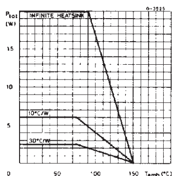
Figure 14. Maximum allowable power dissipation vs. ambient temperature
