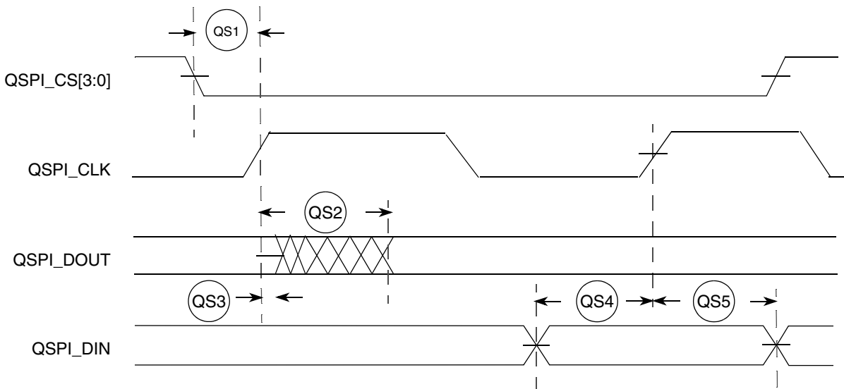
Figure 30. QSPI Timing
