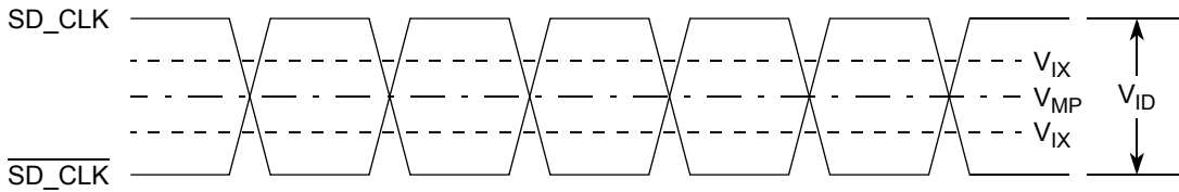
Figure 14. SD_CLK and SD_CLK crossover timing
