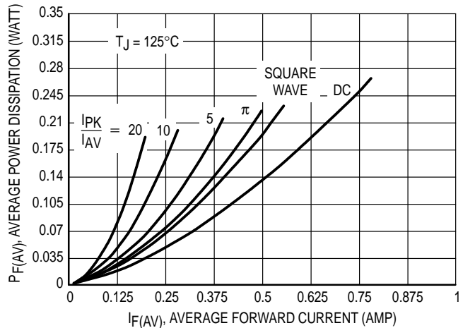
Figure 6. Power Dissipation
