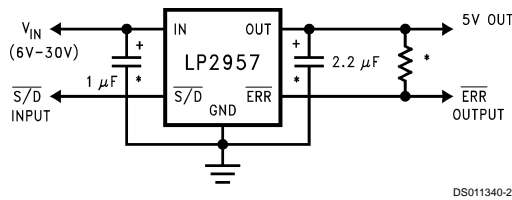
LP2957 Basic Application
