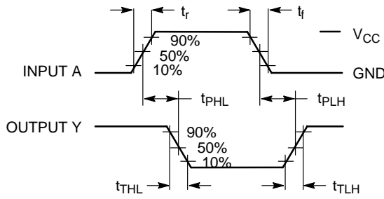
Figure 4. Switching Waveforms
