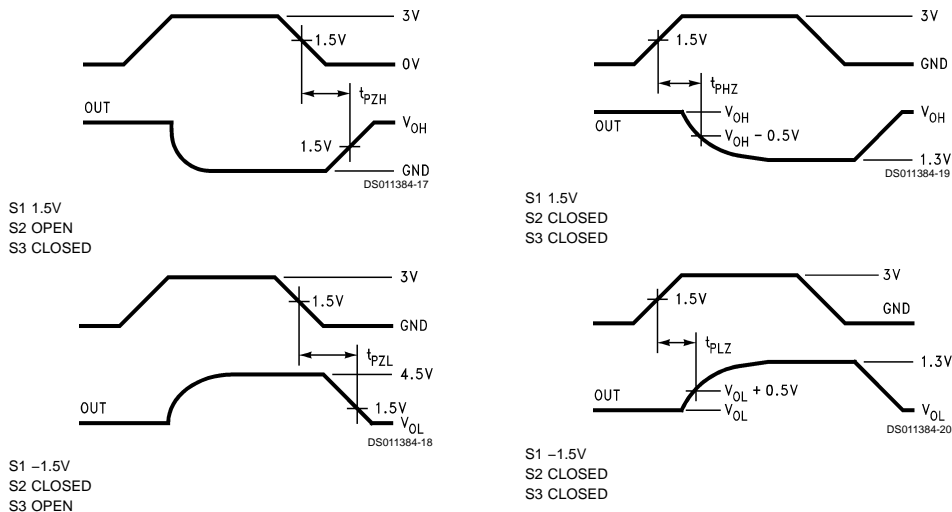
FIGURE 16. Receiver Enable and Disable Timing
