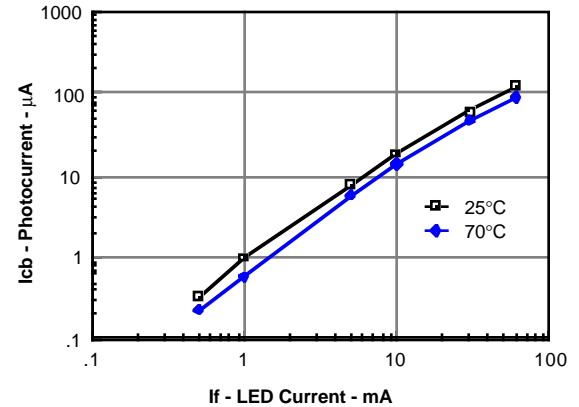
Figure 7. Photocurrent versus LED current
