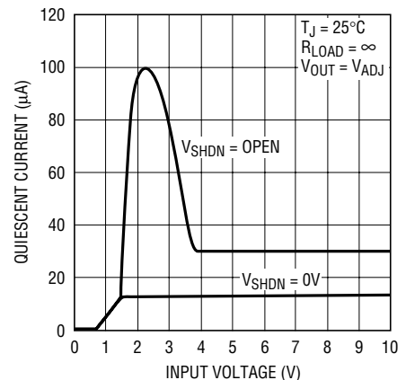
LT1121 Quiescent Current
