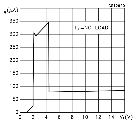
Figure 9 : Quiescent Current vs Input Voltage
