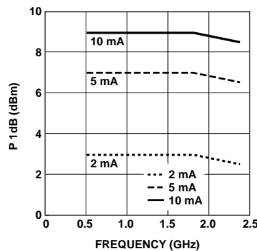
Figure 5. AT-31011 and AT-31033 Power at 1 dB Gain Compression vs. Frequency and Current at V_{\text{CE}} = 2.7\text{ V} .
