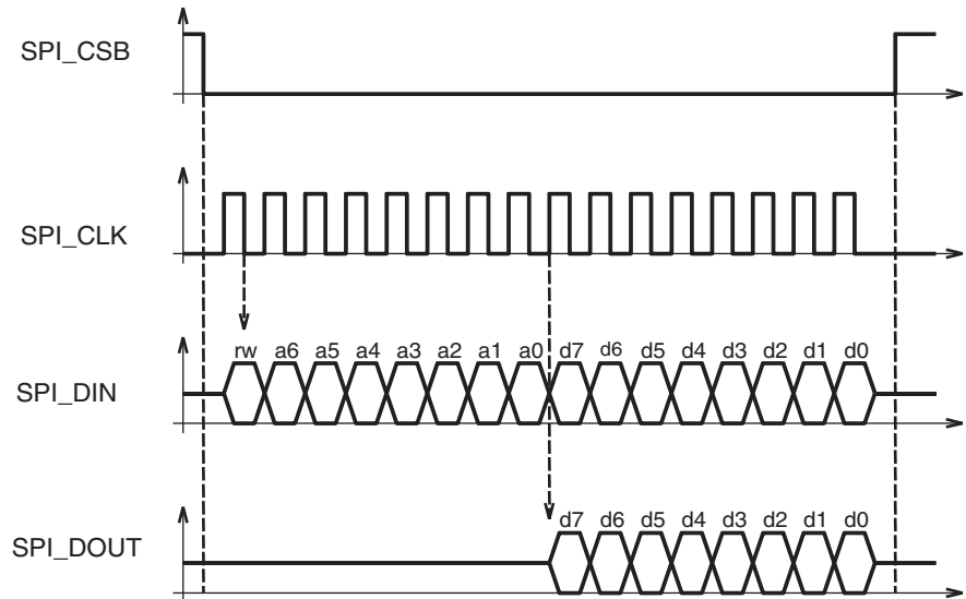
Figure 8-1. SPI Architecture
