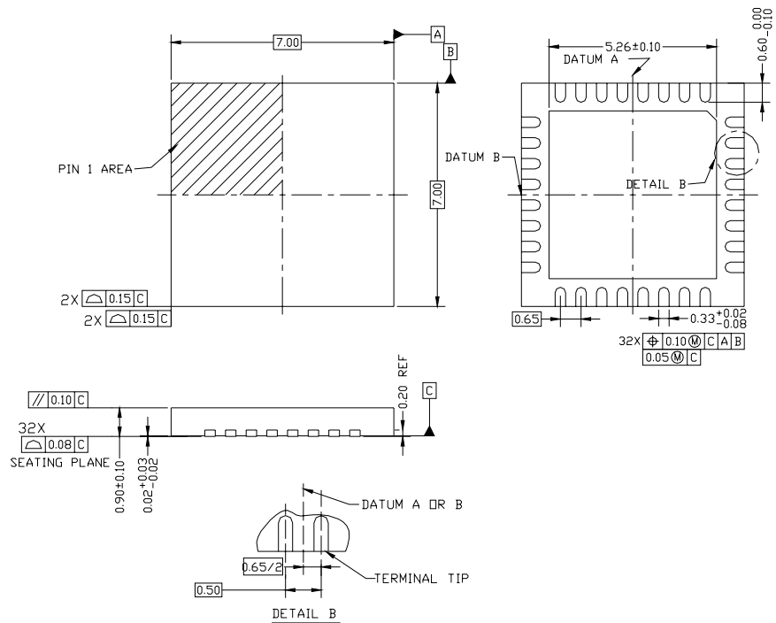
Figure 12-1. Package Outline
