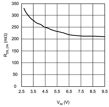
R_{DS(ON)} ( ON ) vs V_{DD}
