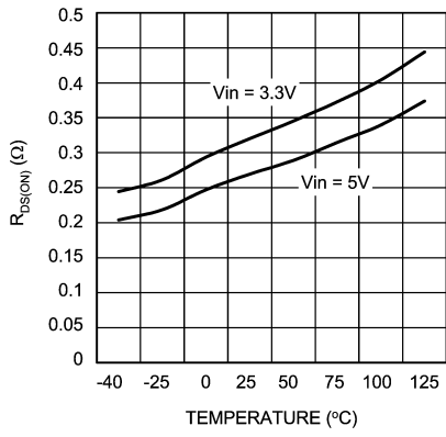
R_{DS(ON)} ( ON ) vs Temperature
