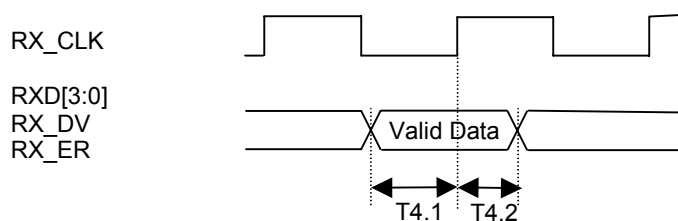
Figure 6.4 10M MII Receive Timing Diagram
