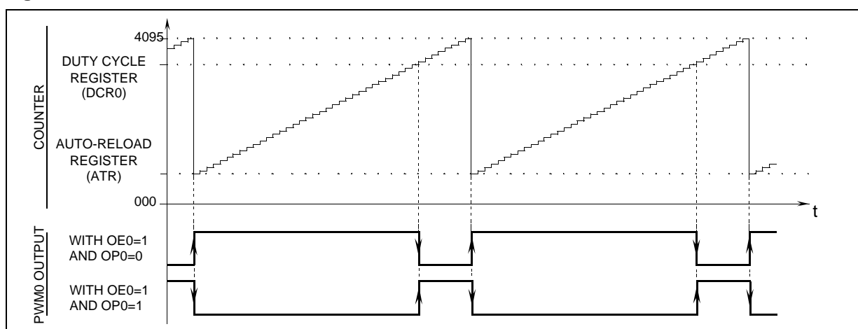
Figure 34. PWM Function
