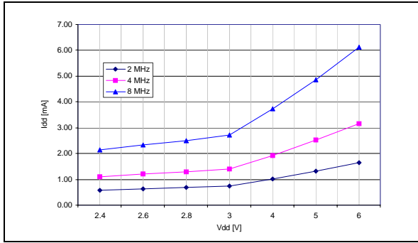
Figure 41. Typical I DD in SLOW vs. f CPU
