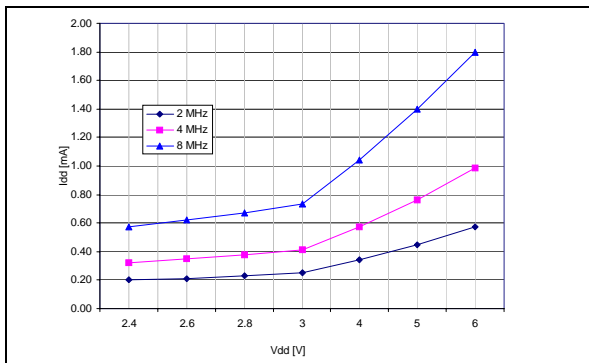
Figure 42. Typical I DD in WAIT vs. f CPU
