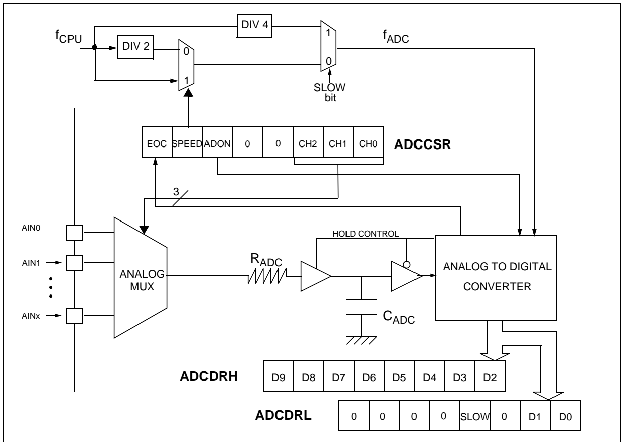
Figure 36. ADC Block Diagram
