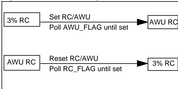
Figure 9. Clock Switching
